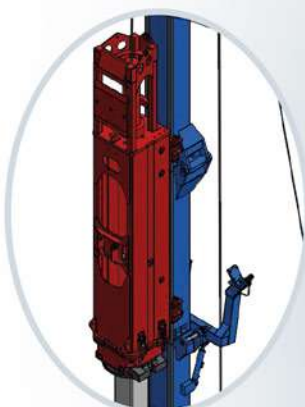
PD Driven Piles
