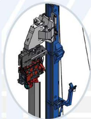
SV Sheet Piles Vibrator
