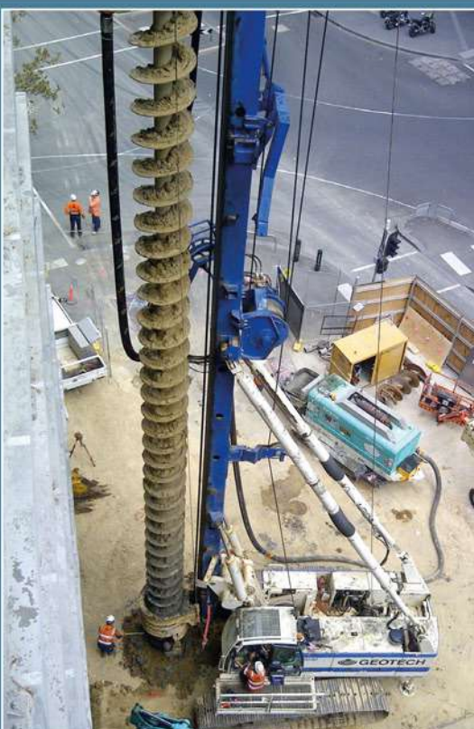
AUSTRALIA E6050 LM - CFA240 CFA Piles.
